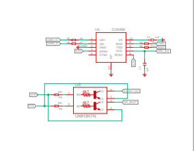
USB TO UART
