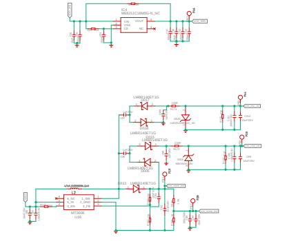
LCD_POWER
